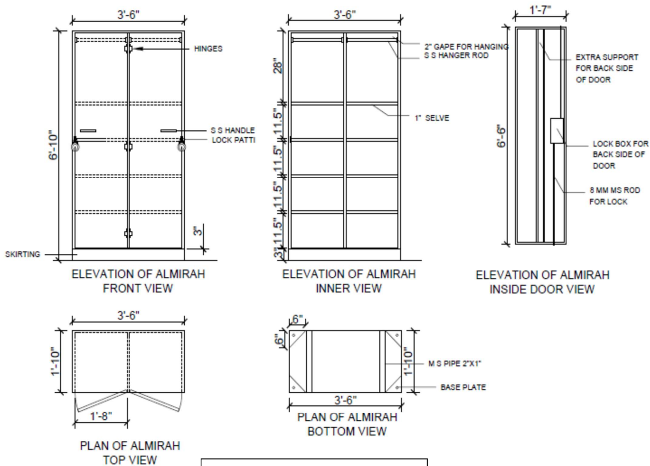
Student Almirah Drawing - 1
