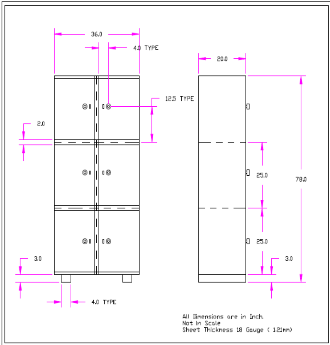
Locker Almirah Drawing - 1
