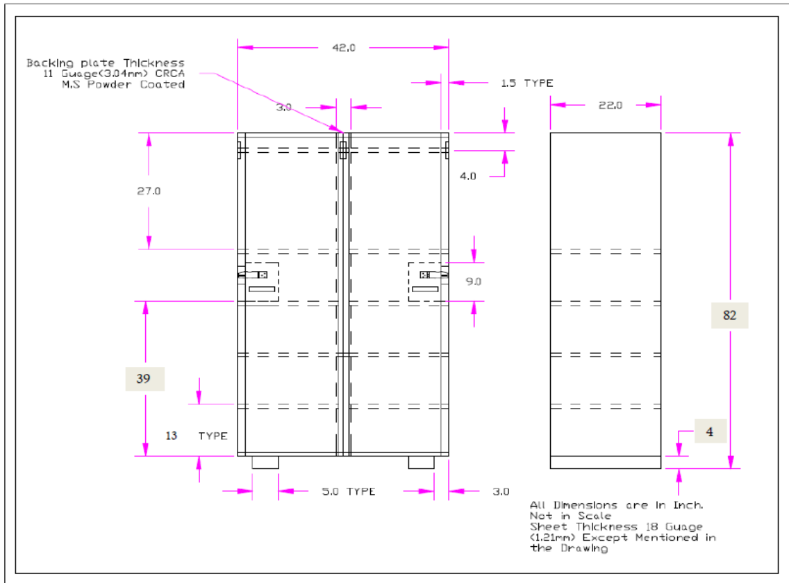
Student Almirah Drawing - 1
